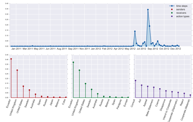
Figure 6: Julian Assange, editor-in-chief of WikiLeaks, sought asylum at the Ecuadorian embassy in the UK during June through August 2012. This component inferred from GDELT (2011 through 2012, with weekly time steps) had the sparsest time-step factor vector. We performed a web search for ecuador UK sweden june 2012 to interpret this component.
